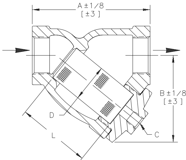
2 [DN50] Strainer Shown Above
